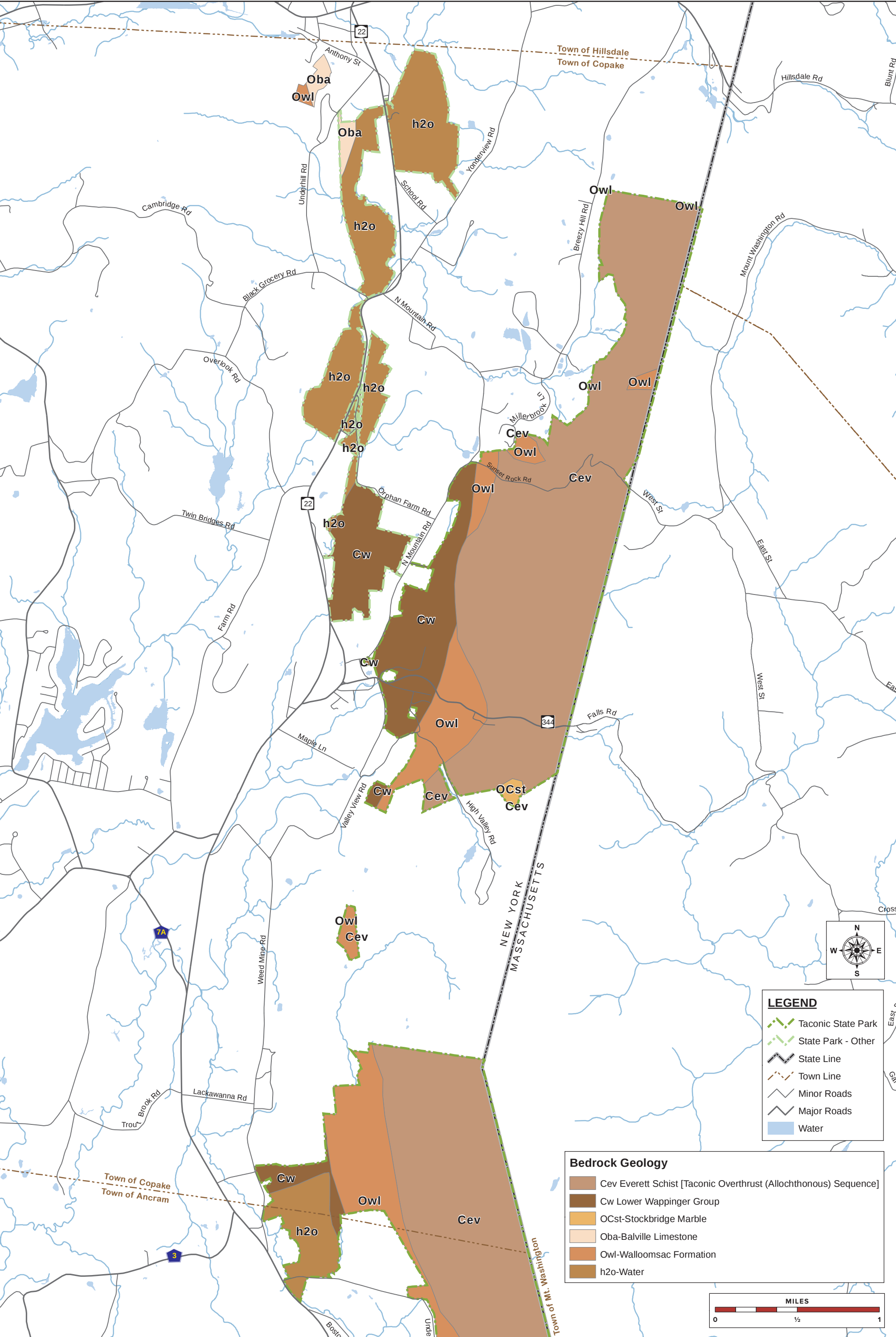
Figure 3A - BEDROCK GEOLOGY NORTHERN SECTION
